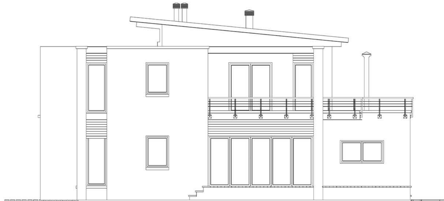
EAST ELEVATION
